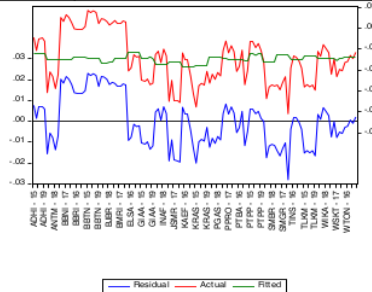
Picture 2 Eviews version 10 (2021) Heteroscedasticity Test Results
