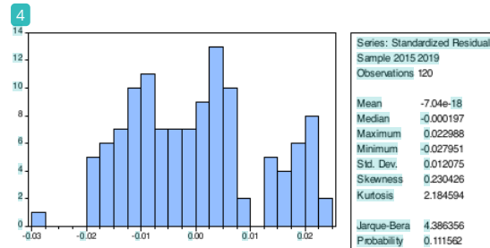
Picture 1 Normality Test Results
